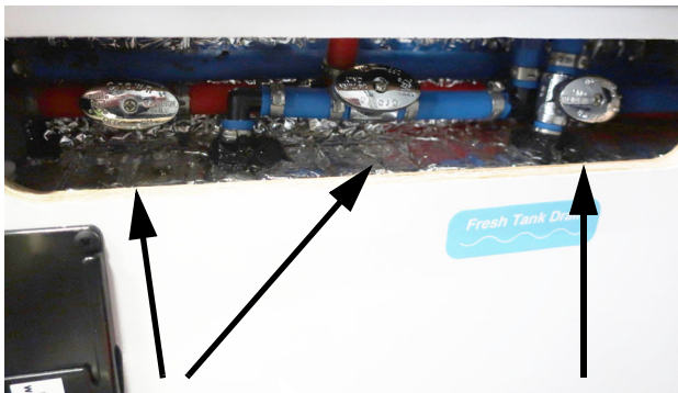
Waterline Drain Valves Fresh Tank Drain Valve Waterline and Fresh Tank Drain Valves -Typical View
